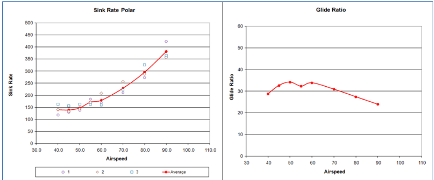
Figure 5 - Sink Rate and Glide Ratio Plots
